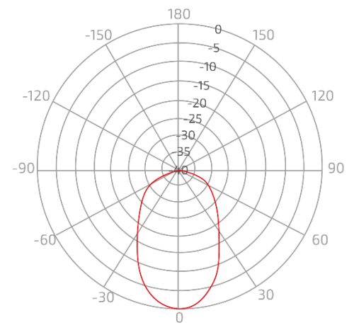
Elevation - SH-5800-18-30-DP
